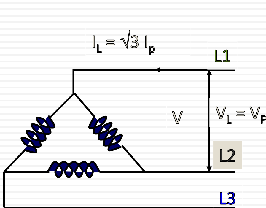
Delta connection
