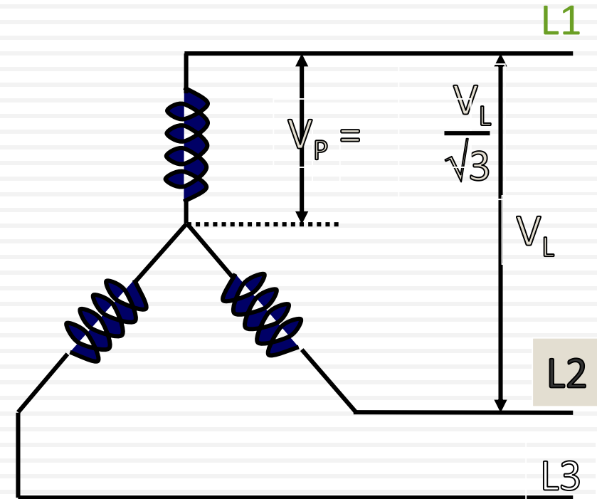
Star connection
